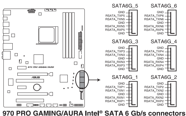
970 PRO GAMING/AURA Intel® SATA 6 Gb/s connectors
